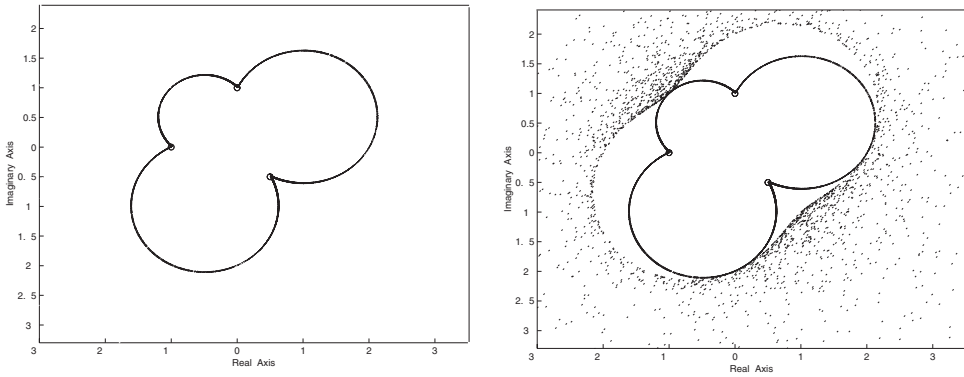
FIGURE 1 The numerical ranges W(A_1\lambda + A_0) and W(B_1\lambda + B_0) .
