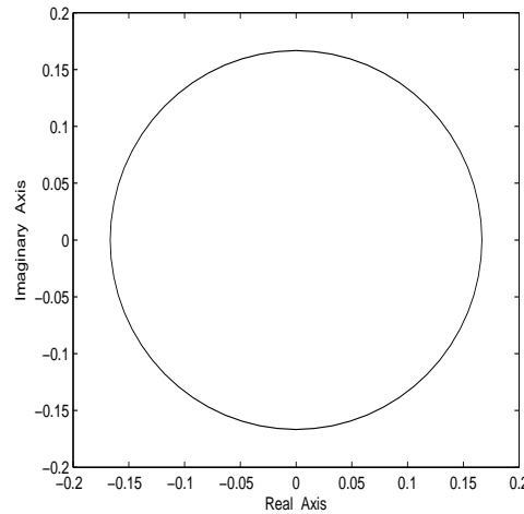
Fig. 3. The numerical range of L^{-1/2}AL^{-1/2} in Example 4.2.
